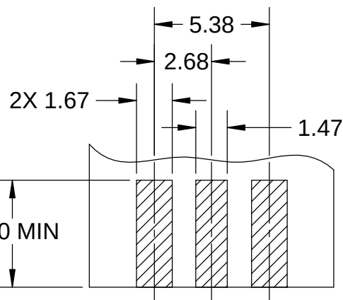
SUGGESTED PCB PAD LAYOUT
