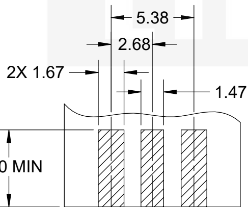
SUGGESTED PCB PAD LAYOUT
